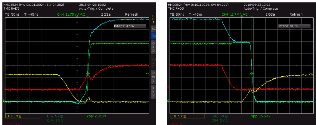
Figure 3.6 Ringing of output (green) and Gate voltages (yellow, blue) with DRVSTRENGTH=0
