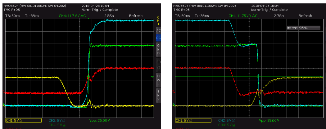
Figure 3.7 Ringing of output (green) and Gate voltages (yellow, blue) with DRVSTRENGTH=2
