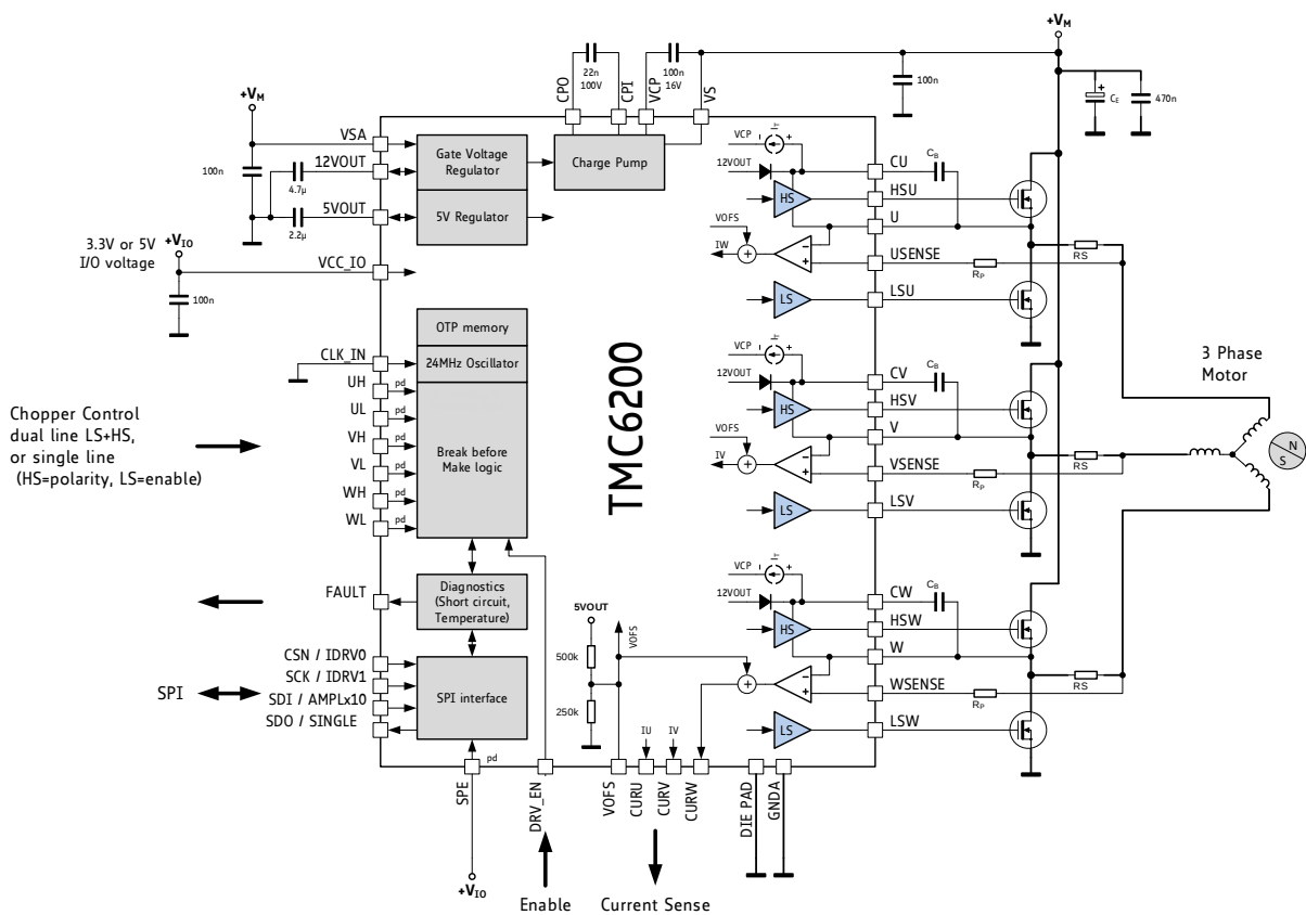
Figure 1.3 SPI mode application
