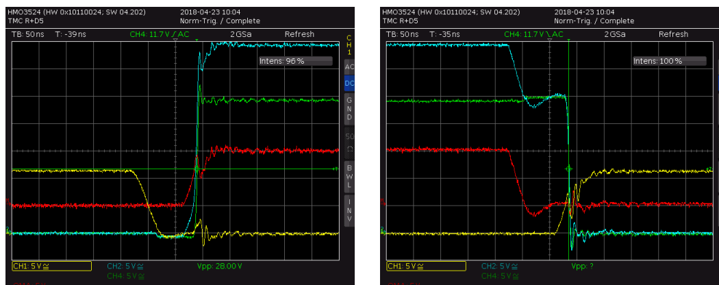
Figure 3.8 Ringing of output (green) and Gate voltages (yellow, blue) with DRVSTRENGTH=3
