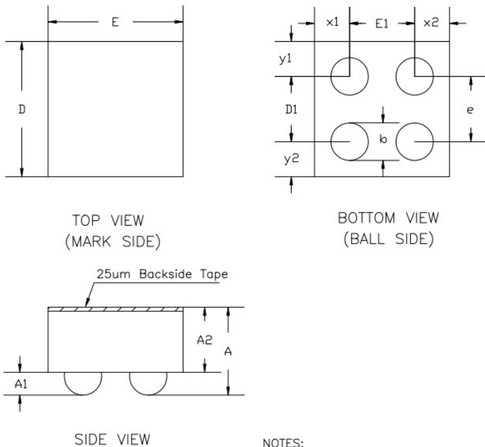
Figure 4. Package Size
