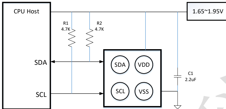
Figure 6. External Connection
