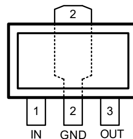
SOT-89-3L AxxPL
