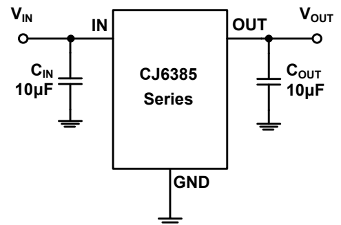
Figure 2-1. Typical Application Circuit
