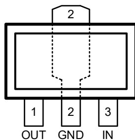
SOT-89-3L AxxPT
