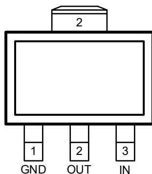
SOT-223 AxxGW
