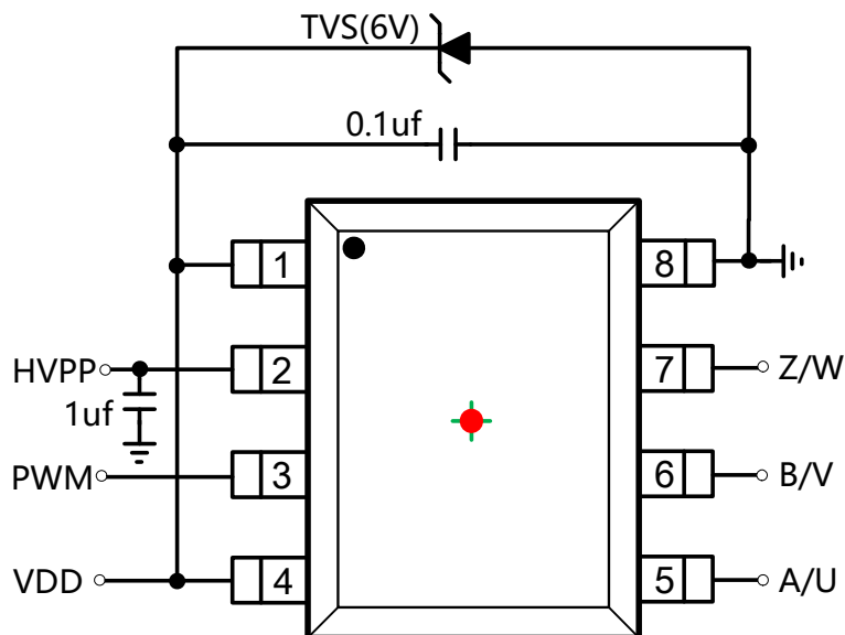
Figure 6: ABZ, UVW and PWM Output Reference Circuit w/i MTP Programming
