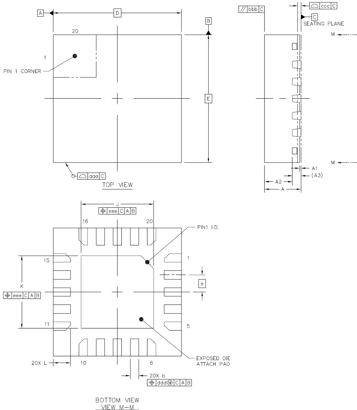
Figure 20.1 Dimensional drawings QFN20
