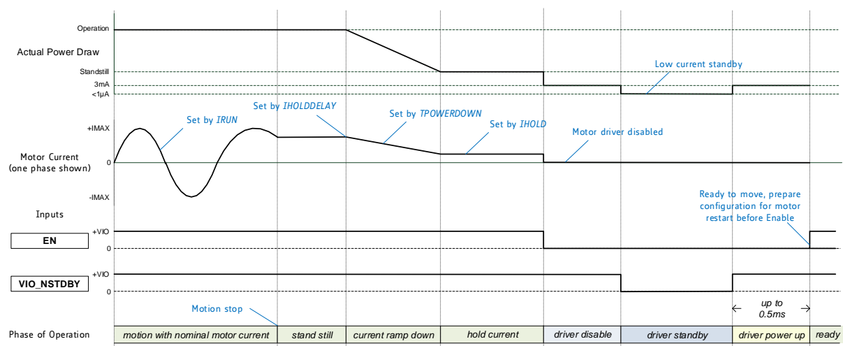
Figure 3.3 Switching to Standby and Back On
