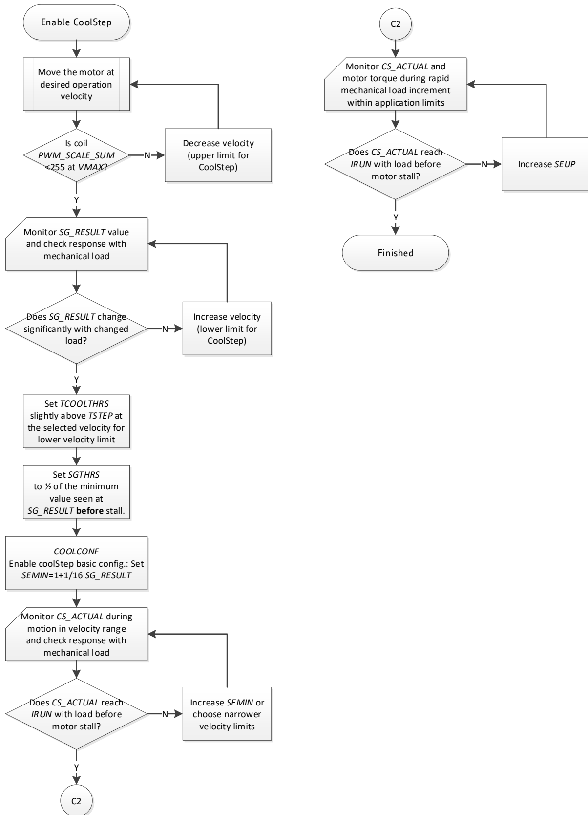
Figure 14.2 Configuration for CoolStep in StealthChop mode
