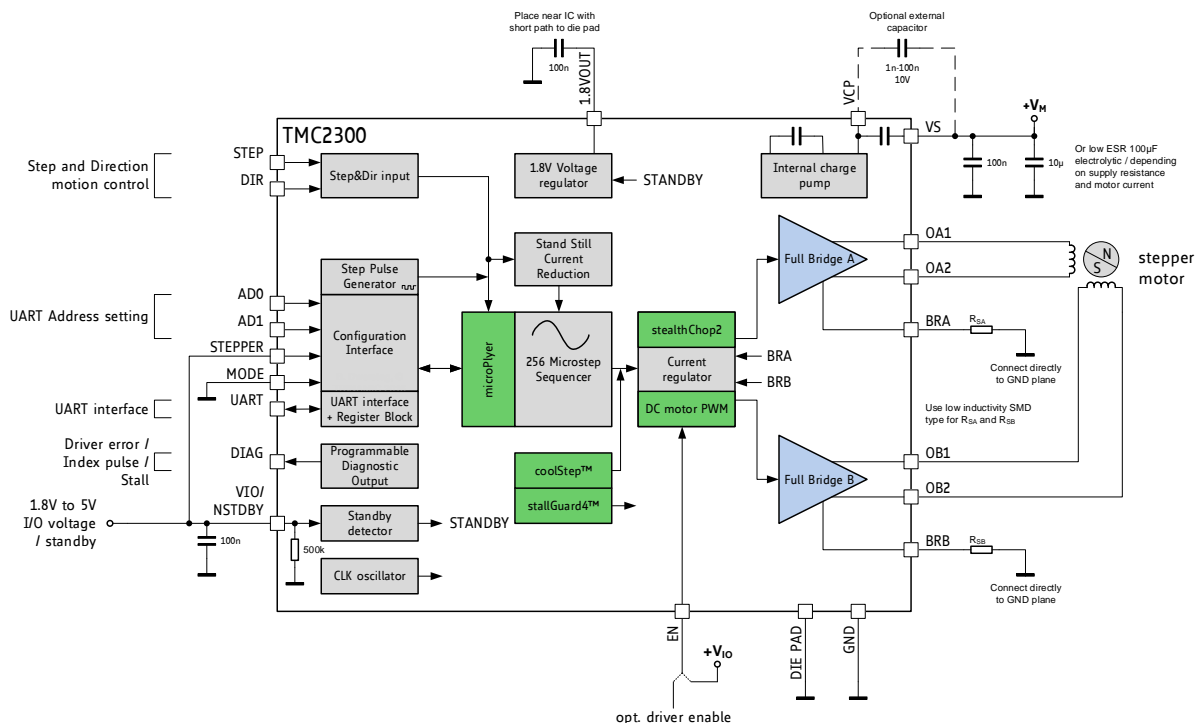
Figure 3.1 Standard Application Circuit for 1.8V to 11V Supply
