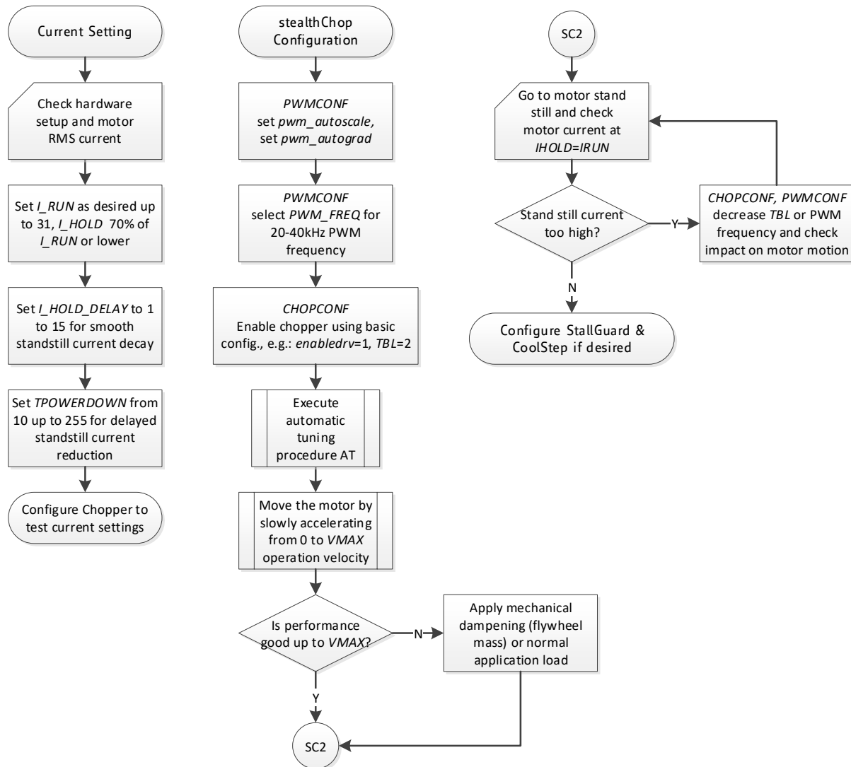
Figure 14.1 Current Setting and Chopper Configuration
