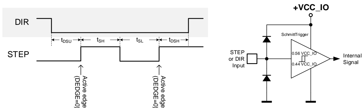
Figure 11.1 STEP and DIR timing, Input pin filter
