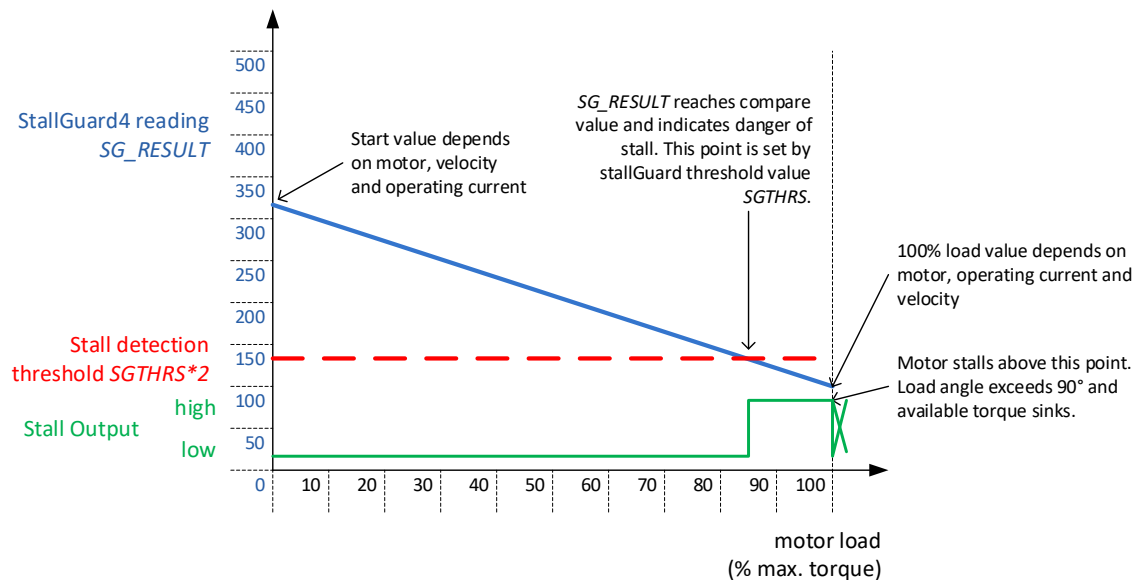
Figure 9.1 Function principle of StallGuard4
